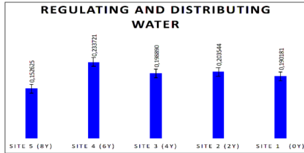
Fig 2: Regulating and distributing water in paddy soil.
